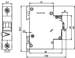
1-pole
