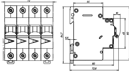
3+N-pole, 4-pole
