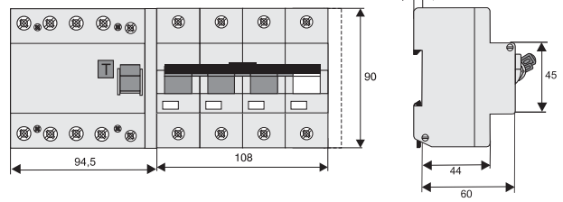
FBHmV/4p + AZ/4p
