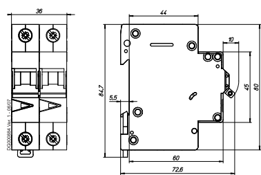
1+N-pole, 2-pole
