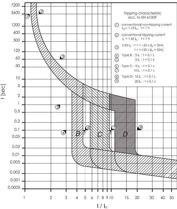
Tripping Characteristic FRBm. 3+N-pole, Characteristics B, C and D
