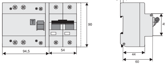
FBHmV/4p + AZ/3p
