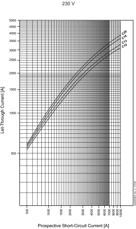
Characteristic C
