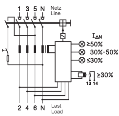
4-pole
