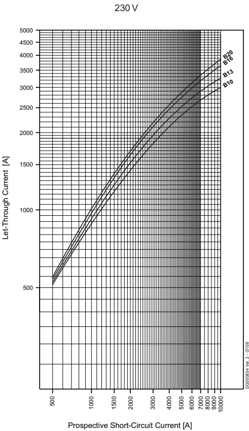
Characteristic B
