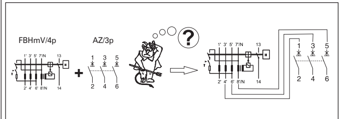
FBHmV-3+N-pole
