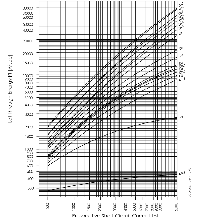
Type D (IEC/EN60947-2)
