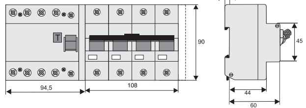
FBHmV/4p + AZ/4p
