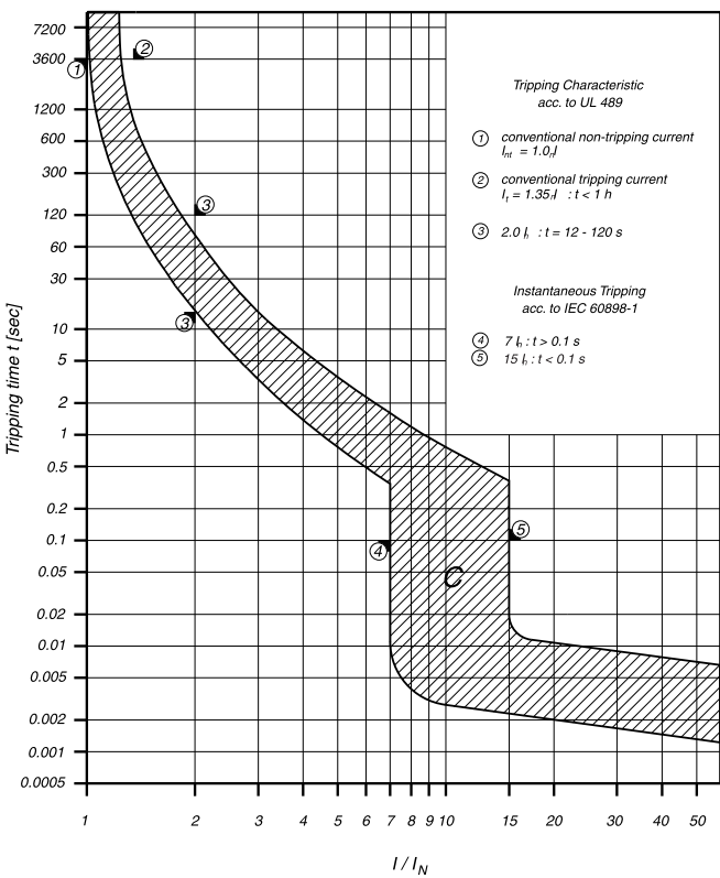
Characteristics C - UL 489
