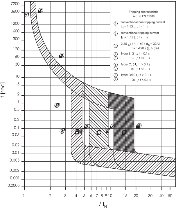
Tripping Characteristic FRBmM 3-pole, Characteristics B, C and D
